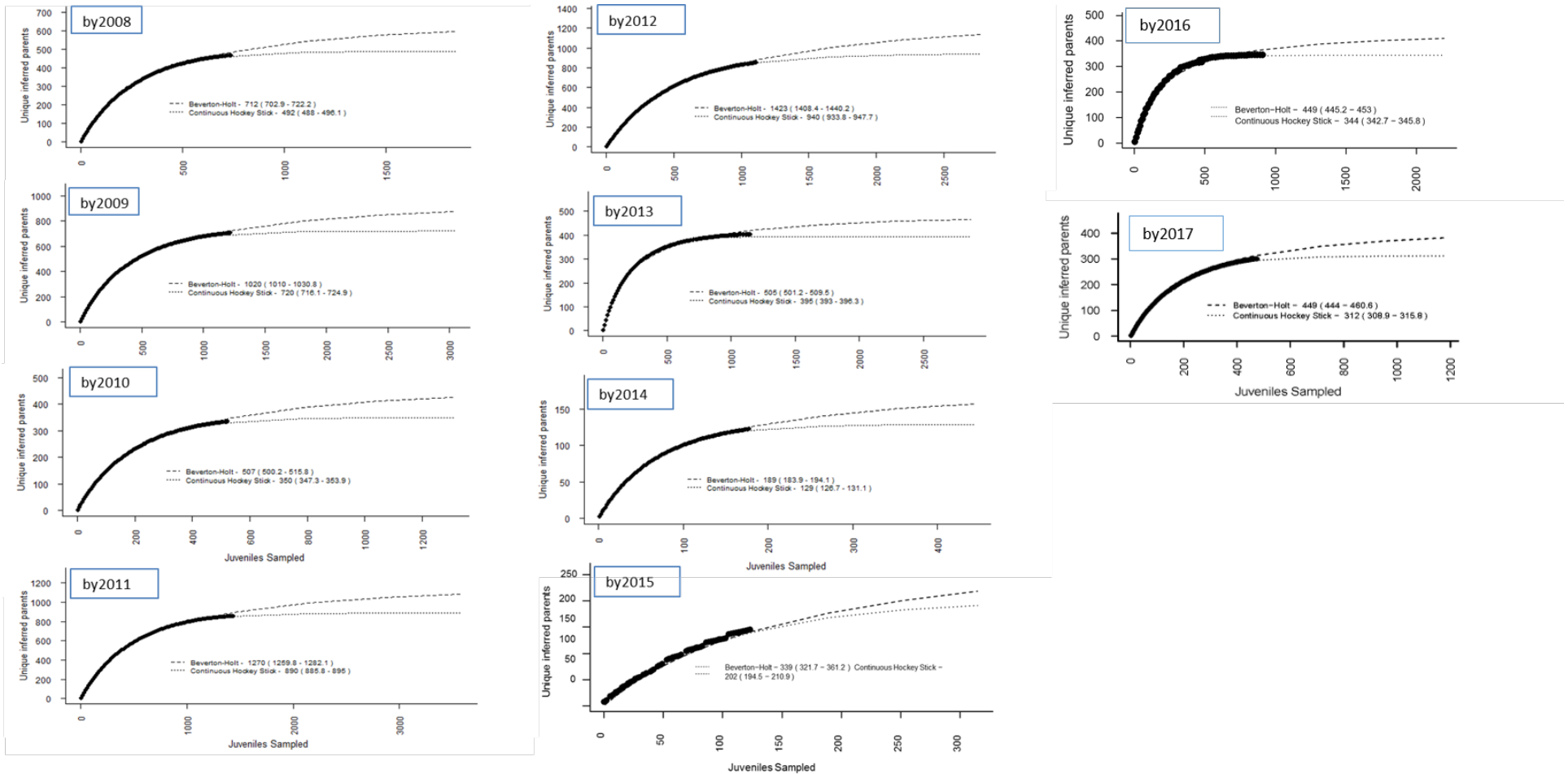
Figure 3. Rarefaction curves estimating spawners in brood years 2008 through 2017. The large dots are the averages over 10,000 re-samples.
