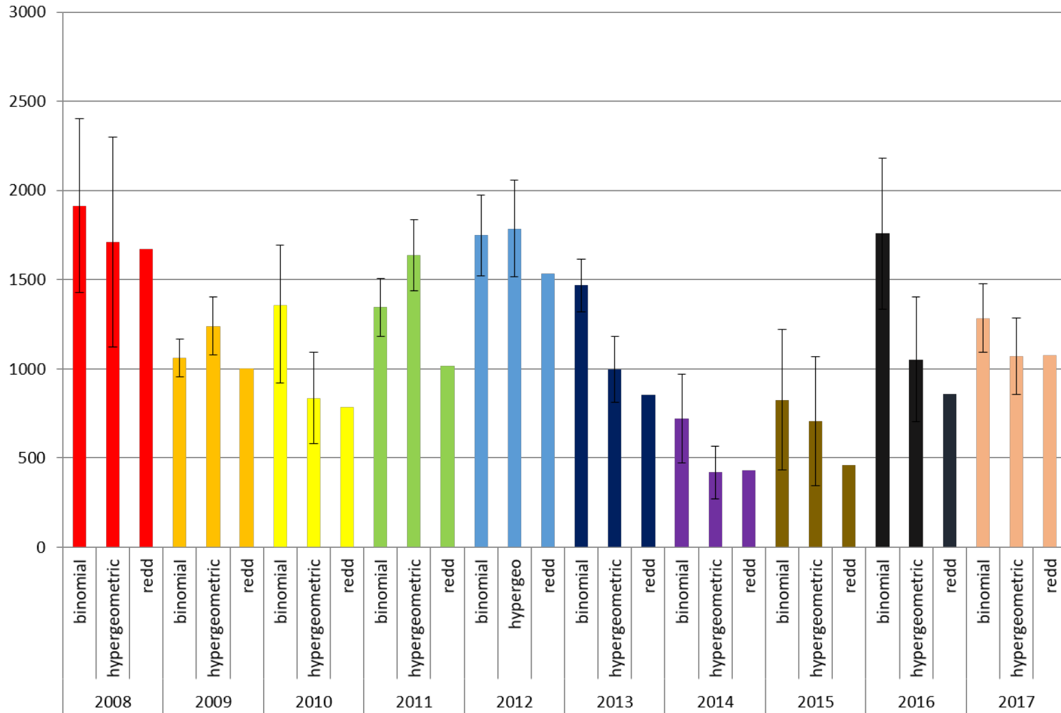
Figure 2. Comparison of the abundance estimates with different methods: binomial, hypergeometric, and redd-based estimate (redd).
