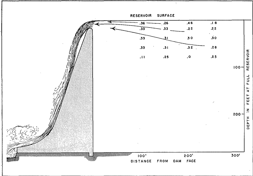
FIGURE 26. Pattern and velocity of flow in front of spillway gates. Three gates full open and two cracked one foot. Velocities shown in feet per second. Discharge 4650 cfs.
