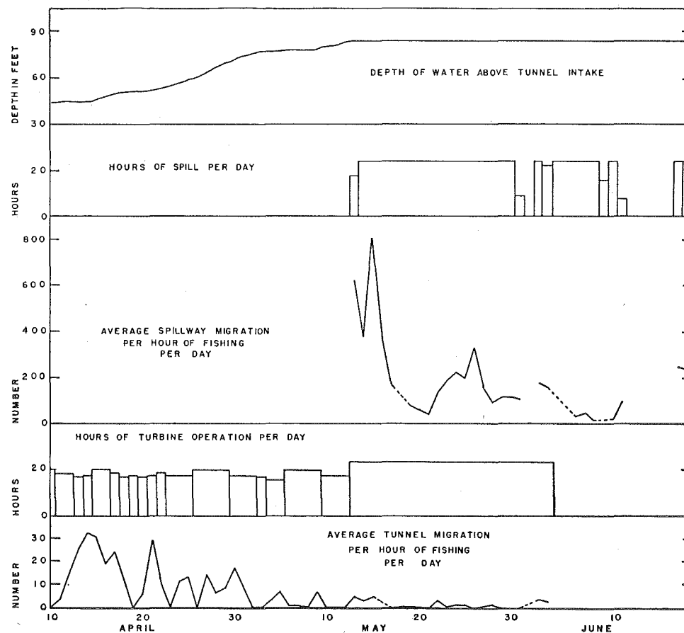
FIGURE 10. Calculated number of coho passing per hour over the spillway and through the turbines in 1952. Period of spill and plant operation also shown. Depth of tunnel intake shown in upper graph.
