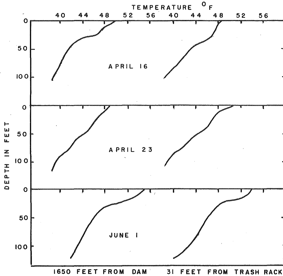
FIGURE 24. Reservoir temperatures taken 1650 feet upstream from the dam and 31 feet in front of the tunnel intake in 1951.
