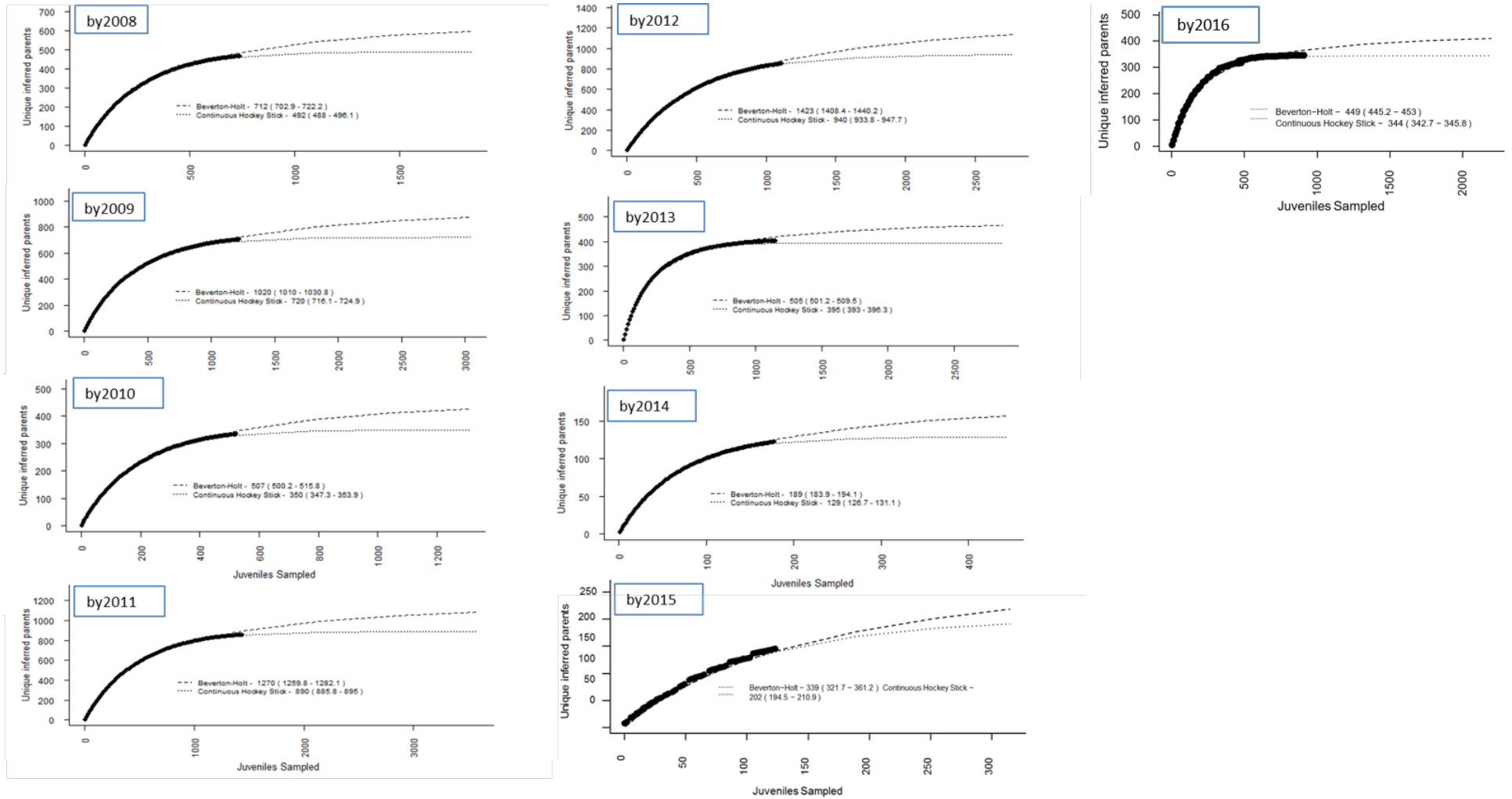
Figure 3. Rarefaction curves estimating spawners in brood years 2008 through 2016. The large dots are the averages over 10,000 re-samples.
