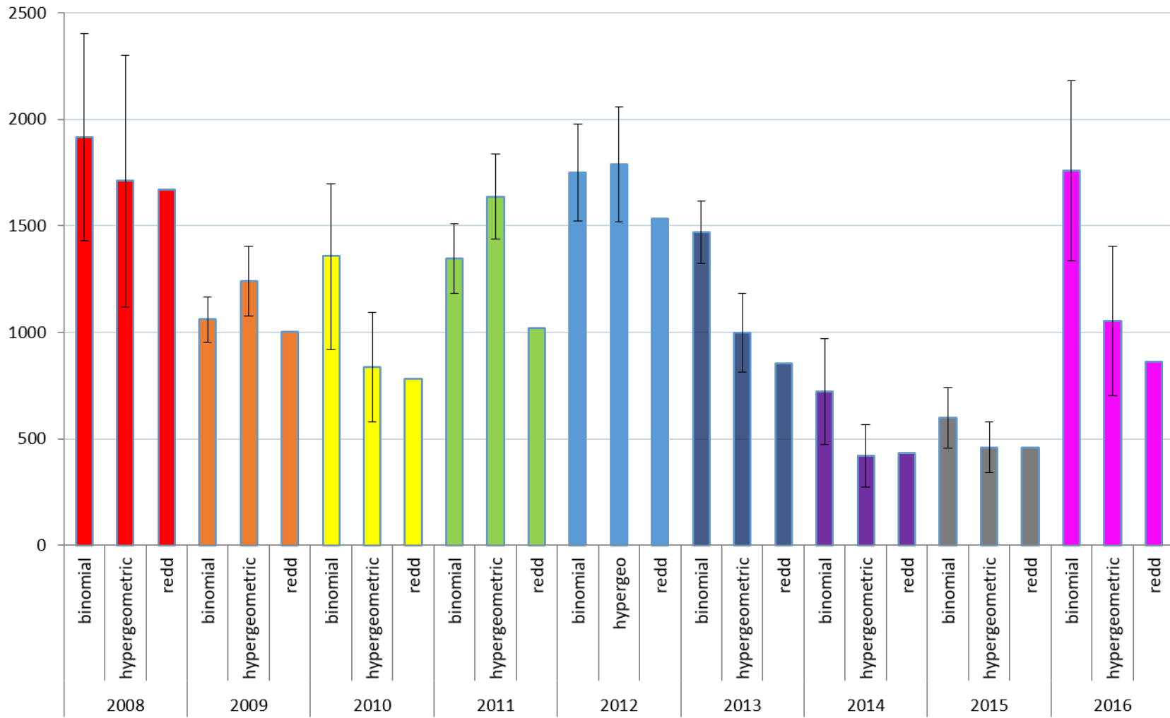
Figure 2. Comparison of the abundance estimates with different methods: binomial, hypergeometric, and redd-based estimate (redd).
