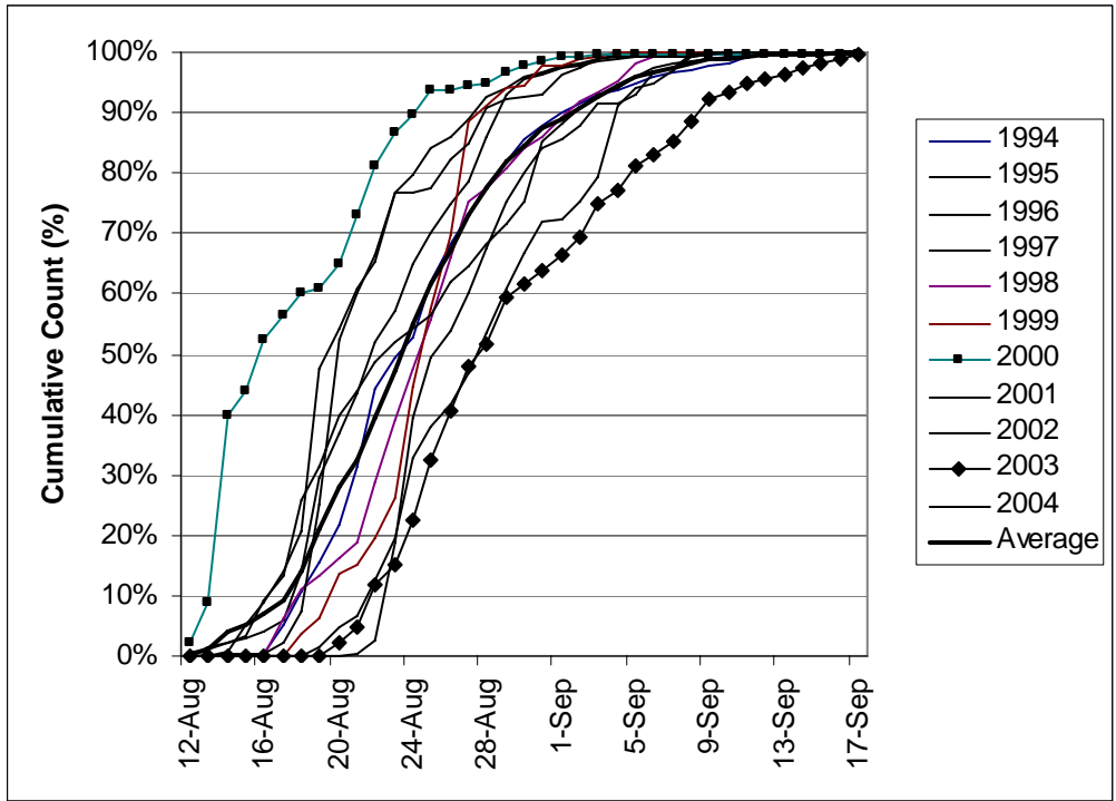
Figure 3. Cumulative count of sockeye at Scotch Creek fence, 1994-2004.
