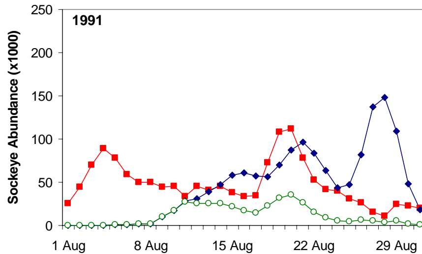
Appendix Figure B1. Daily estimates of arriving Summer-run and Late-run Sockeye, and of Late-run escapement (left panels); and daily estimates of the number of sockeye present in the Gulf, including the arriving Summer-run and Late-run sockeye, and the resident Late-run fish (right panels). Note that the Y axis range for 1998 and 2002 differs from that for other years.
