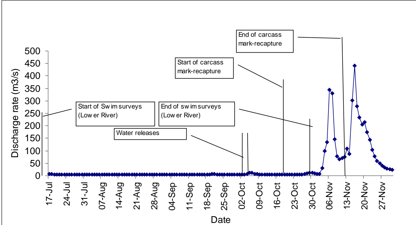
Figure 3. Daily Nanaimo River Discharge (m 3 /s) during the fall run chinook season, 2006. Discharge data are preliminary and subject to revision
