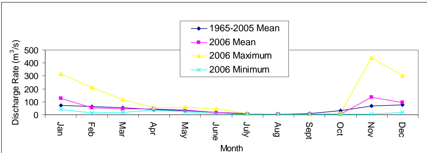
Figure 4. Monthly Nanaimo River discharge (m 3 /s) in 2006 along with historic (1965-2005) mean.
