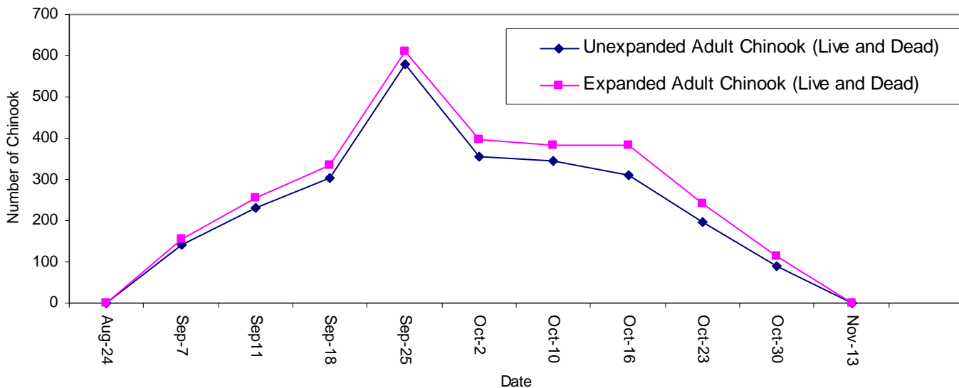
Figure 5. Expanded (for observer efficiency) and unexpanded swim survey counts, lower Nanaimo River, 2006.
