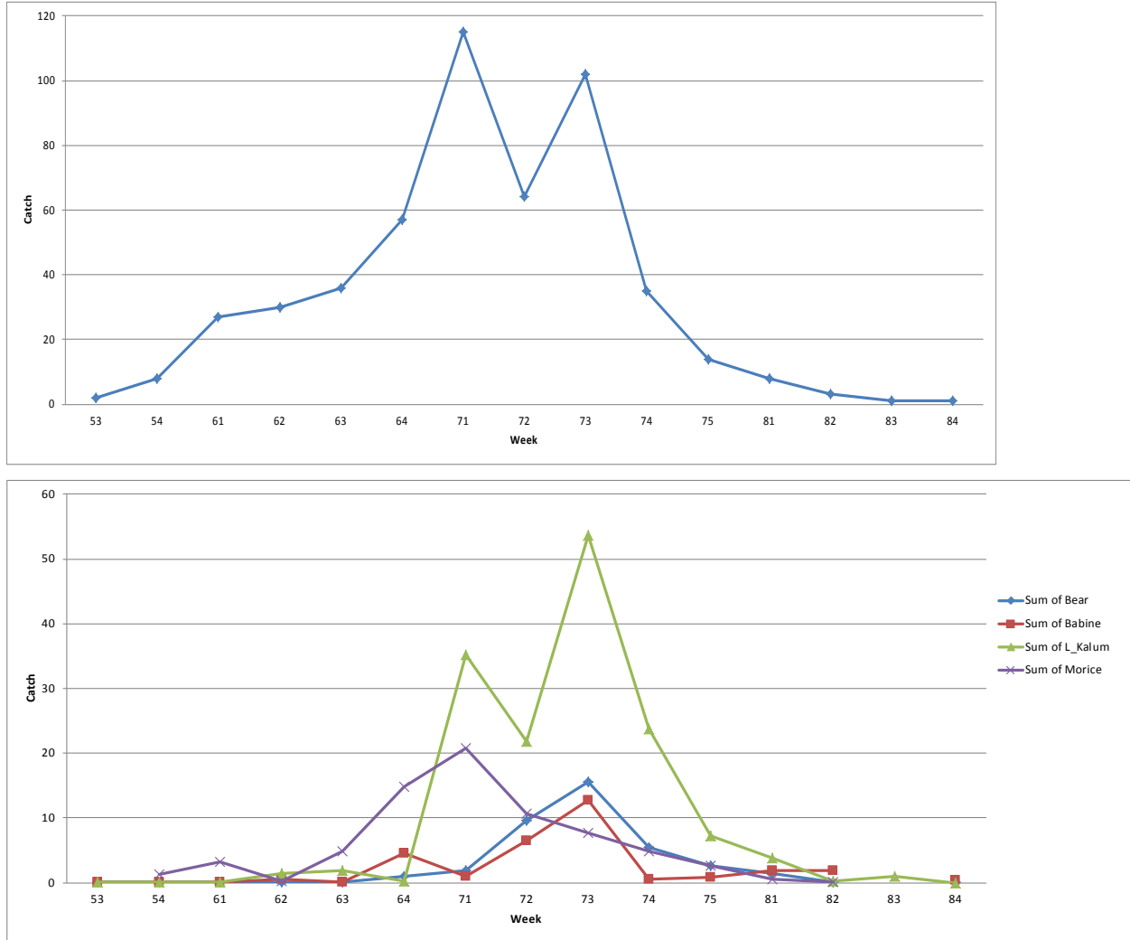
Figure 4. Total catch of Chinook salmon and catch of Chinook salmon from large component stocks at the 2013 Tye Test Fishery by week.
